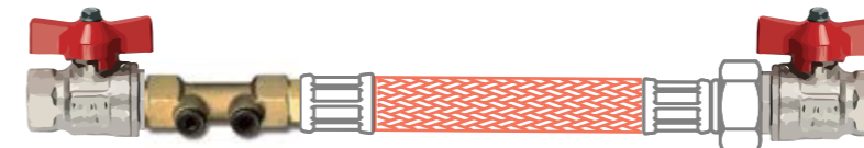
Filler loop EA GALVA FF DN13 braided in galvanized steel. With EA backflow 1/2" and *T* ball valves 1/2"FF
